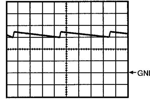
WF13 1DIV: 2V 5msec
