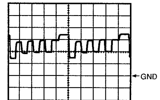
WF20 1DIV: 50V 10 μsec
