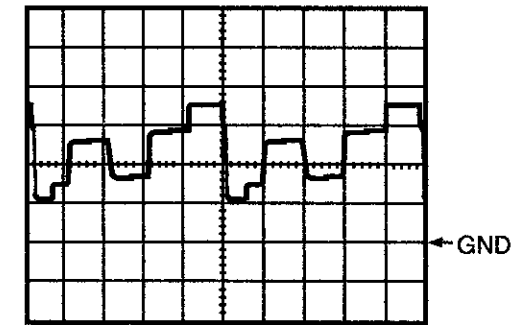
WF18 1DIV: 50V 10 μsec
